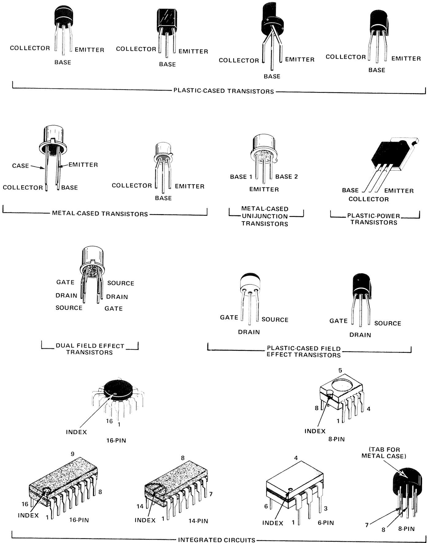
Fig. 6-1. Semiconductor lead configurations.
