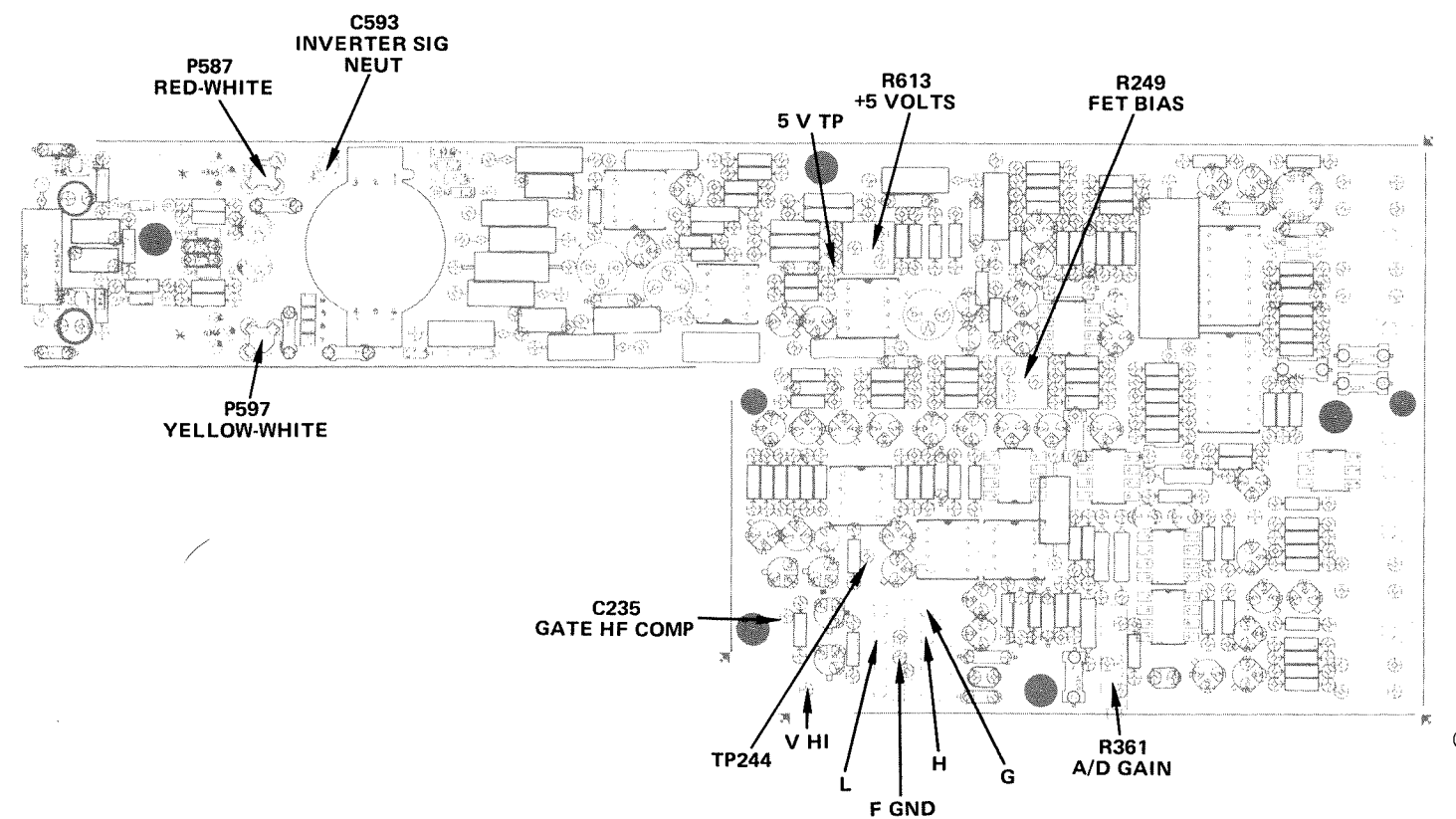
Fig. 6-8. (A2) Floating circuit board adjustment locations.
