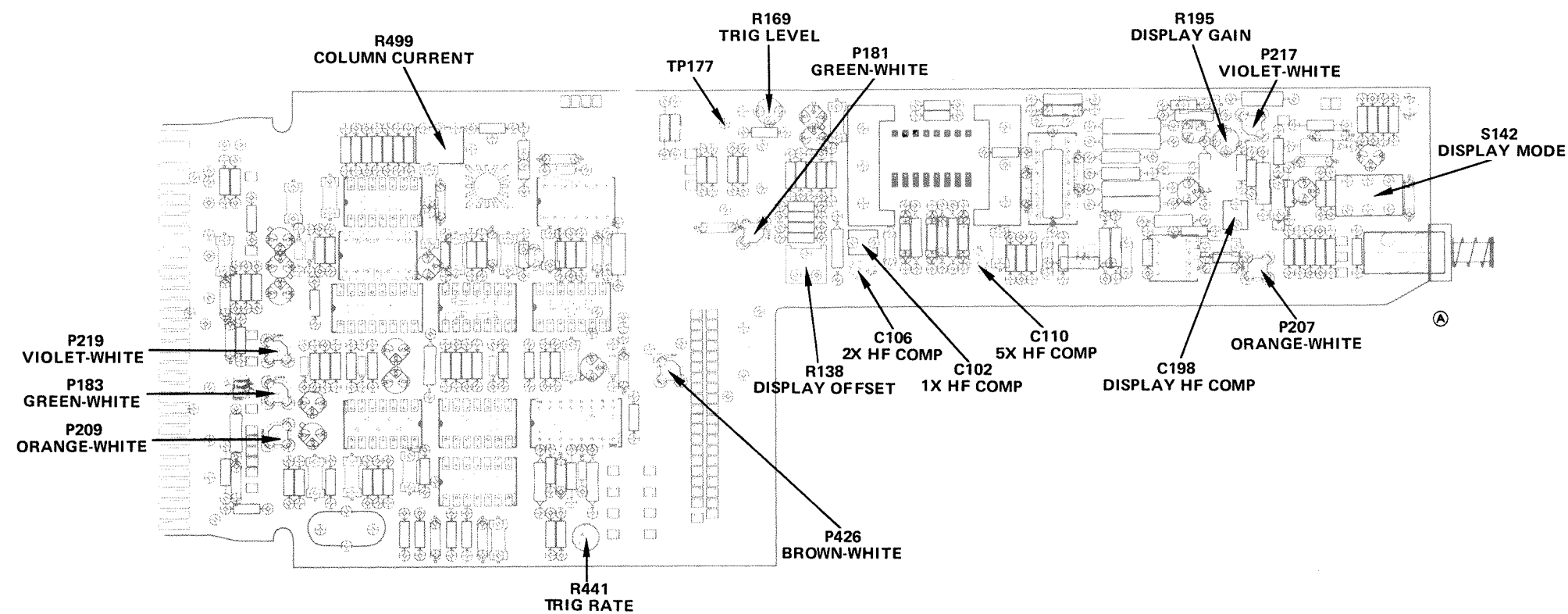
Fig. 6-7. (A1) Main circuit board adjustment locations.
